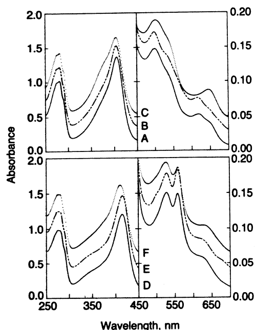
FIG. 2. Optical spectra of wild-type and mutant CCP in the native and compound ES states. Samples were prepared by dissolving crystals of the appropriate enzyme in 100 mM sodium phosphate buffer (pH 6.0) to a concentration of \approx 10 \mu\text{M} . The samples were filtered ( 0.45 \mu\text{m} ), and spectra were collected at 15^\circ\text{C} . Compound ES was generated by addition of hydrogen peroxide to a final concentration of 50 \mu\text{M} immediately before the spectra were recorded. (Upper) Spectra for native enzyme containing Met-172 (spectrum A), Cys-172 (spectrum B), and Ser-172 (spectrum C). (Lower) Compound ES spectra for enzymes containing Met-172 (spectrum D), Cys-172 (spectrum E), and Ser-172 (spectrum F). Spectra B, C, E, and F are offset for clarity.
